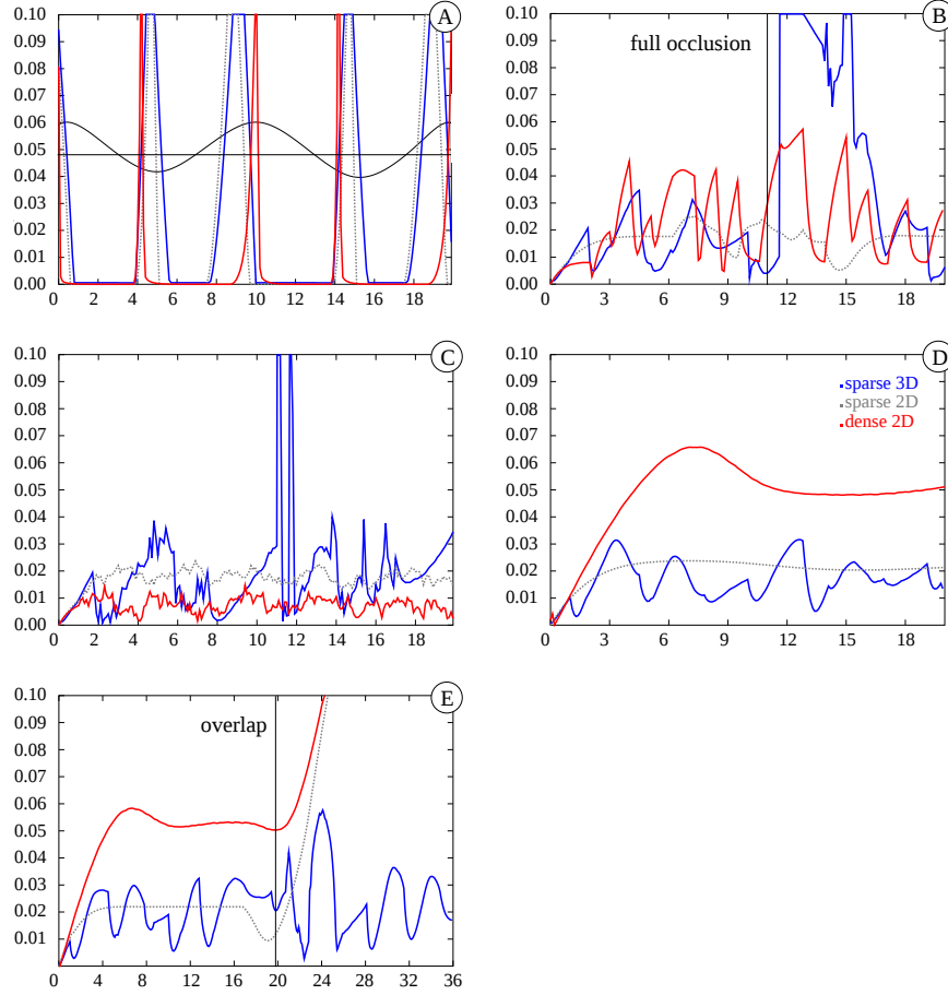
Fig. 7 Error distance as a function of time for scenarios A to E for three different implementations: 2D dense (plain red), 2D sparse (dashed), 3D sparse (plain blue). All error distances are clamped in [0, 0.1] as divergence generally occurs when above (up to a distance of 0.4 on the manifold). The black lines for scenario A represent the 2 stimuli intensity as a function of time, while they represent peculiar events for scenario B and E.
