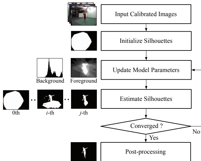
Fig. 1: Approach Outline: first silhouettes are initialized with the projection of the camera visibility domain; Then background and foreground model are iteratively updated and silhouette are re-estimated at each iteration using both color and spatial consistency constraints. Once the optimization is completed, a post-processing step is performed to refine the estimated silhouettes.
