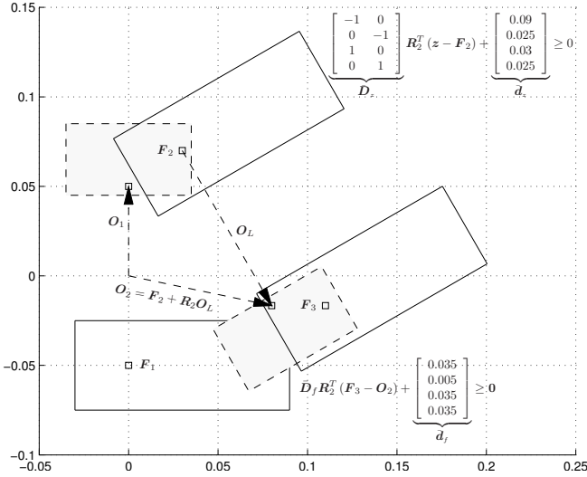
Fig. 1. Constraints on the ZMP and position of the feet. \mathbf{F}_i \in \mathbb{R}^2 and \mathbf{R}_i \in \mathbb{R}^{2 \times 2} define the position (of a point of interest) and orientation of foot i relative to the world frame. \mathbf{O}_L is an offset defining the position of (a point of interest of) the constraint for foot i + 1 relative to foot i (expressed in the local frame fixed in foot i ).
