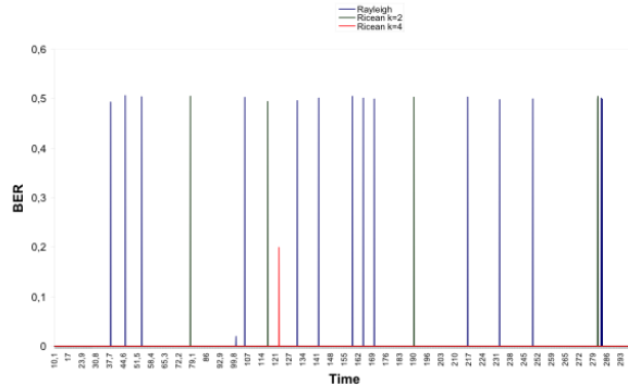
Figure 18: PLP0-Dist 100km - BER vs Simulated time
