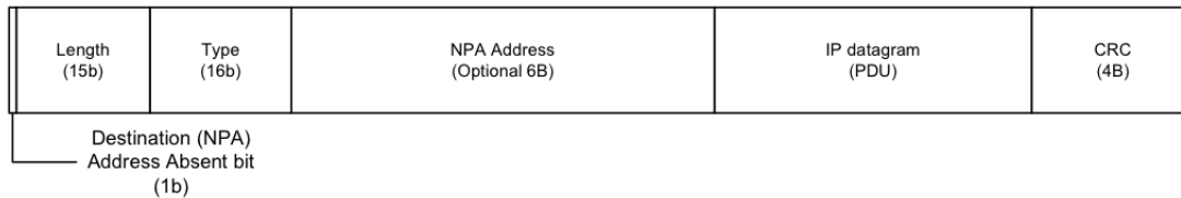
Figure 6: ULE packet format
