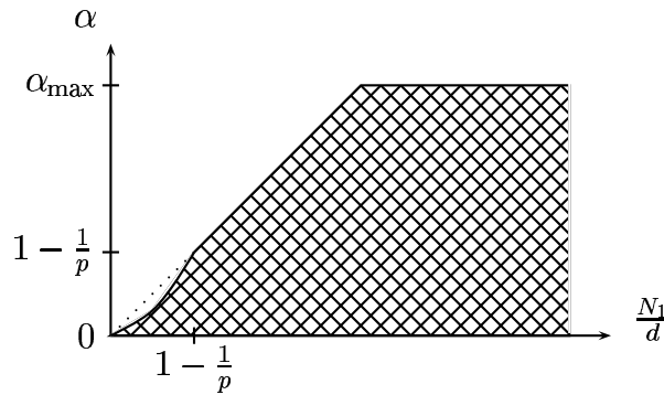
FIGURE 1. A crosshatch of the range of admissible values of \alpha in Theorem 6.1 (given by (6.1)) as a function of N_1/d , \alpha_{\max} = \min\{s/d, \gamma/d - 1/p\} .
