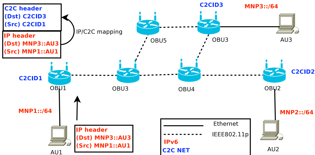
Figure 6: in-vehicle network discovery
