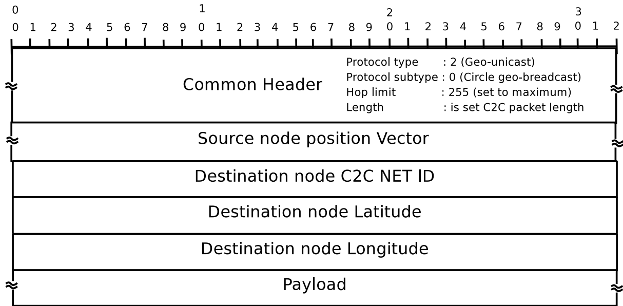
Figure 2: Geo-unicast packet
