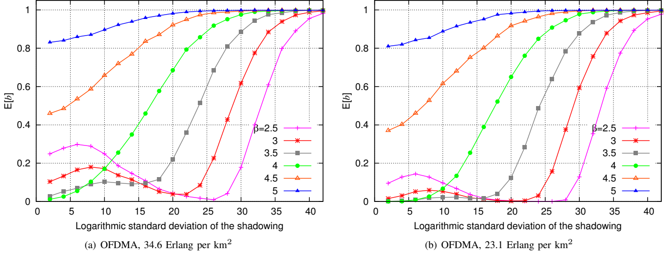
Fig. 3. Blocking probability for OFDMA network as on Figure 2 with traffic 34.6 Erlang per \text{km}^2 and 23.1 Erlang per \text{km}^2 .
