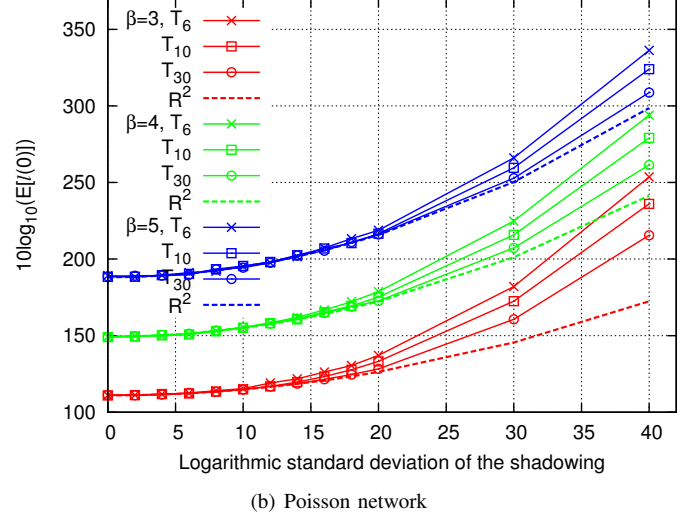
Fig. 5. Mean path-loss factor expressed in dB, in hexagonal and Poisson network on the torus \mathbb{T}_N with log-normal shadowing with log-SD v and path-loss exponent \beta . Note that \mathbb{E}[l(0)] decreases with the size of the network. The analytical expression for the infinite (on \mathbb{R}^2 ) Poisson model is given in Proposition 5.6.
