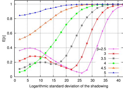
Fig. 2. Blocking probability in OFDMA hexagonal network on the torus \mathbb{T}_6 with log-normal shadowing with log-SD v and path-loss exponent \beta , evaluated using the Kaufman-Roberts algorithm for the traffic 46.2 Erlang per \text{km}^2 .
