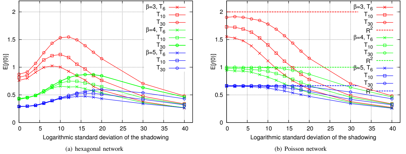
Fig. 4. Mean interference factor in hexagonal and Poisson network on the torus \mathbb{T}_N with log-normal shadowing with log-SD v and path-loss exponent \beta . Note that E[f(0)] increases with the size of the network. The straight lines correspond to the infinite (on \mathbb{R}^2 ) Poisson model; cf. Proposition 5.6.
