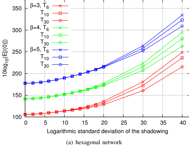
Fig. 5. Mean path-loss factor expressed in dB, in hexagonal and Poisson network on the torus \mathbb{T}_N with log-normal shadowing with log-SD v and path-loss exponent \beta . Note that \mathbb{E}[l(0)] decreases with the size of the network. The analytical expression for the infinite (on \mathbb{R}^2 ) Poisson model is given in Proposition 5.6.
