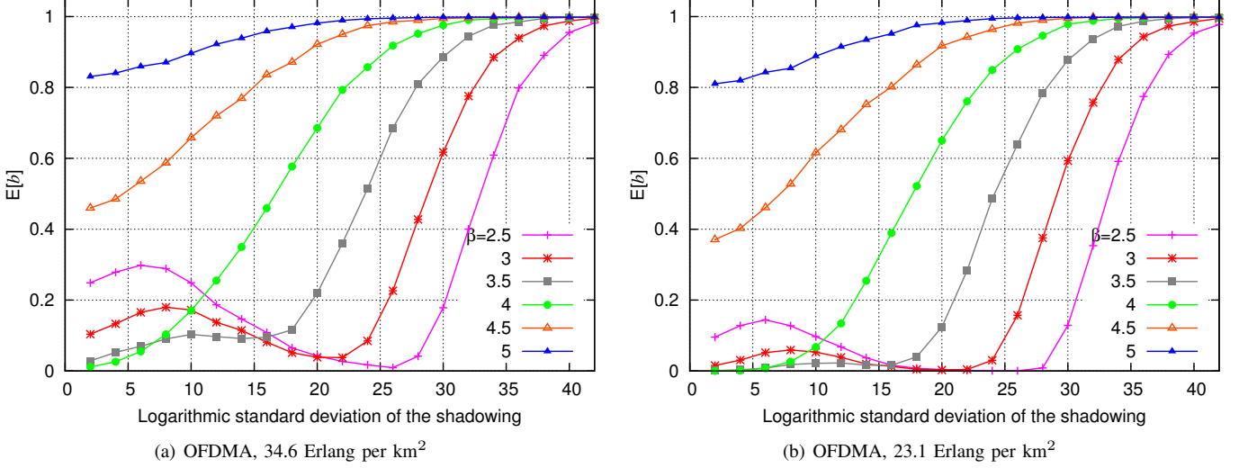
Fig. 3. Blocking probability for OFDMA network as on Figure 2 with traffic 34.6 Erlang per \text{km}^2 and 23.1 Erlang per \text{km}^2 .
