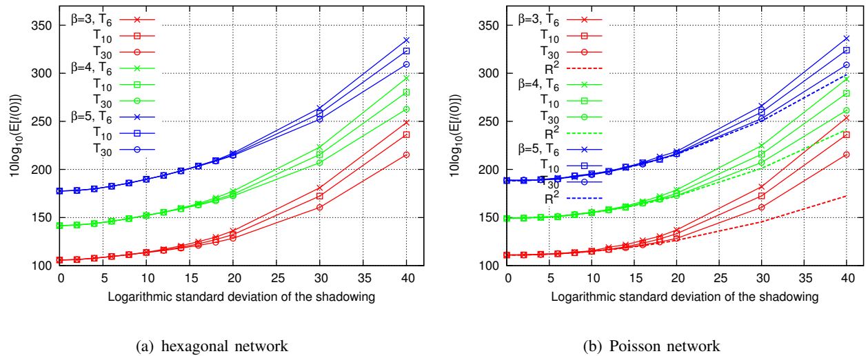
Fig. 5. Mean path-loss factor expressed in dB, in hexagonal and Poisson network on the torus \mathbb{T}_N with log-normal shadowing with log-SD v and path-loss exponent \beta . Note that \mathbb{E}[l(0)] decreases with the size of the network. The analytical expression for the infinite (on \mathbb{R}^2 ) Poisson model is given in Proposition 5.6.
