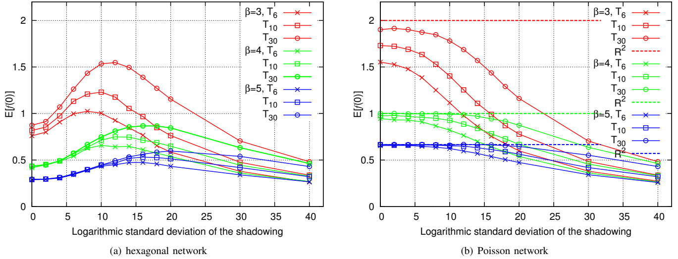
Fig. 5. Mean interference factor in hexagonal and Poisson network on the torus \mathbb{T}_N with log-normal shadowing with log-SD v and path-loss exponent \beta . Note that \mathbb{E}[f(0)] increases with the size of the network. The straight lines correspond to the infinite (on \mathbb{R}^2 ) Poisson model; cf. Proposition 5.5.
