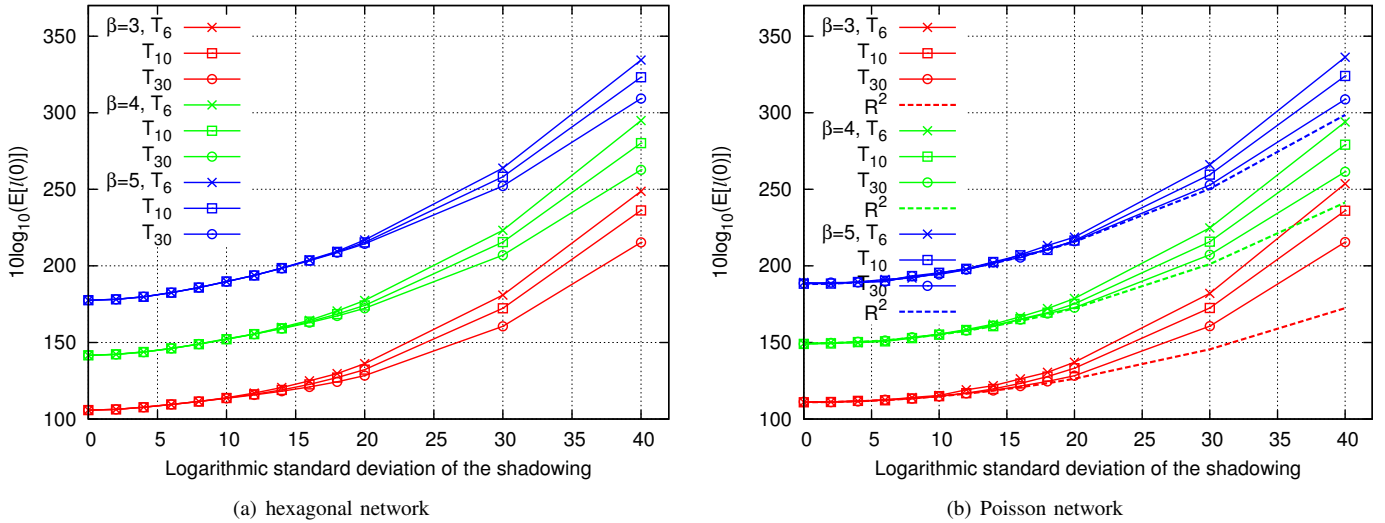
Fig. 6. Mean path-loss factor expressed in dB, in hexagonal and Poisson network on the torus \mathbb{T}_N with log-normal shadowing with log-SD v and path-loss exponent \beta . Note that \mathbb{E}[l(0)] decreases with the size of the network. The analytical expression for the infinite (on \mathbb{R}^2 ) Poisson model is given in Proposition 5.5.
