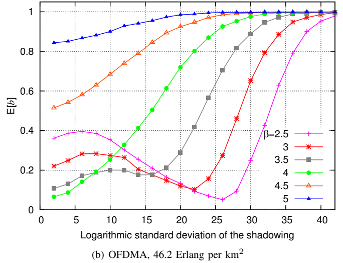
Fig. 2. Blocking probability in CDMA and OFDMA hexagonal network on the torus \mathbb{T}_6 with log-normal shadowing with log-SD v and path-loss exponent \beta , evaluated using the Kaufman-Roberts algorithm for the traffic 46.2 Erlang per km 2 .
