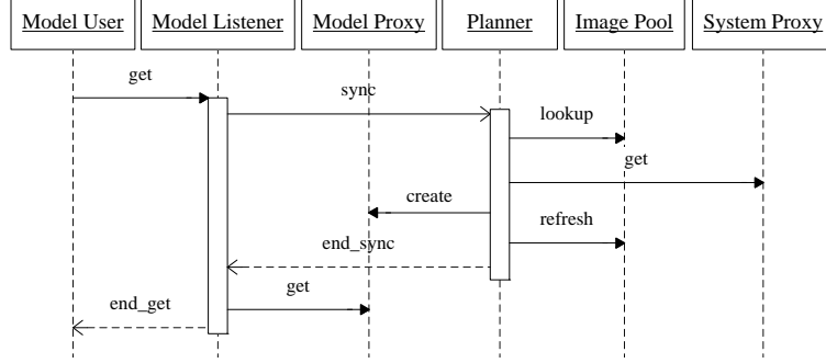
Fig. 6. A sample behavior of the synchronizers
