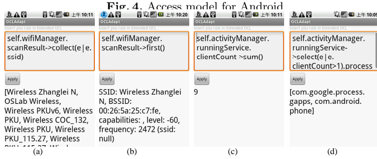
Fig. 5. Android screen shots
