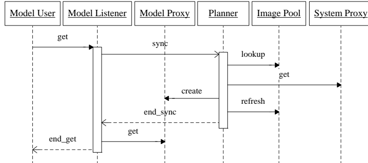
Fig. 6. A sample behavior of the synchronizers
