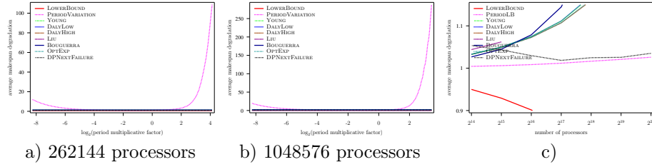
Figure 59: Evaluation of the different heuristics on a Exascale platform with Weibull failures ( MTBF = 1250 years), using Numerical Kernel law with \gamma = 1 , and constant overhead model
