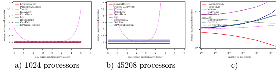
Figure 39: Evaluation of the different heuristics on a Petascale platform with Weibull failures ( MTBF = 500 years), using Amdahl law with \gamma = 10^{-6} , and constant overhead model
