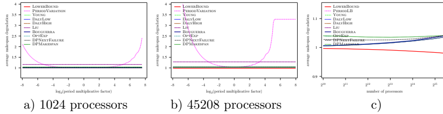
Figure 29: Evaluation of the different heuristics on a Petascale platform with Exponential failures ( MTBF = 500 years), using Numerical Kernel law with \gamma = 0.1 , and constant overhead model
