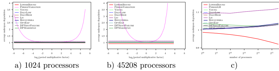
Figure 22: Evaluation of the different heuristics on a Petascale platform with Exponential failures ( MTBF = 125 years) using embarrassingly parallel job, and constant overhead model
