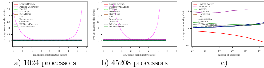
Figure 30: Evaluation of the different heuristics on a Petascale platform with Exponential failures ( MTBF = 125 years), using Numerical Kernel law with \gamma = 1 , and constant overhead model
