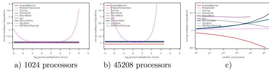
Figure 37: Evaluation of the different heuristics on a Petascale platform with Weibull failures ( MTBF = 500 years), using Amdahl law with \gamma = 10^{-4} , and constant overhead model
