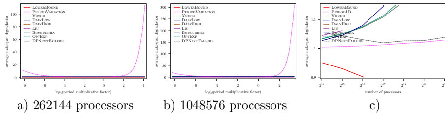
Figure 58: Evaluation of the different heuristics on a Exascale platform with Weibull failures ( MTBF = 1250 years), using Numerical Kernel law with \gamma = 0.1 , and constant overhead model
