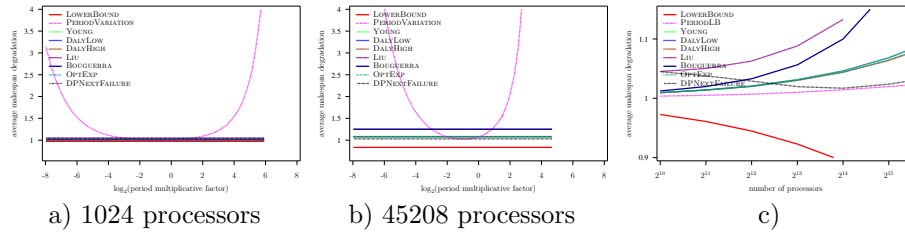
Figure 40: Evaluation of the different heuristics on a Petascale platform with Weibull failures ( MTBF = 125 years), using Numerical Kernel law with \gamma = 0.1 , and constant overhead model
