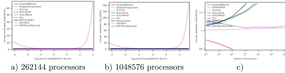
Figure 60: Evaluation of the different heuristics on a Exascale platform with Weibull failures ( MTBF = 1250 years), using Numerical Kernel law with \gamma = 10 , and constant overhead model
