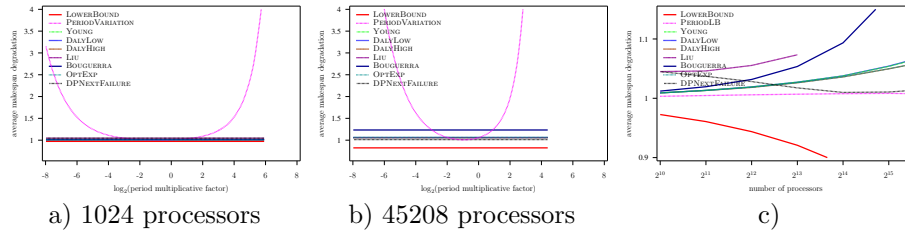
Figure 36: Evaluation of the different heuristics on a Petascale platform with Weibull failures ( MTBF = 125 years), using Amdahl law with \gamma = 10^{-4} , and constant overhead model
