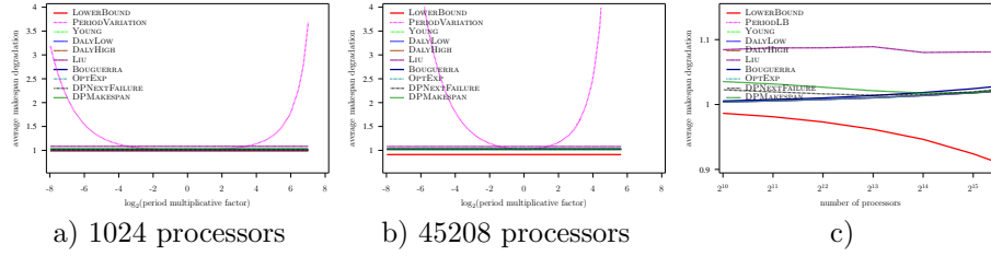
Figure 32: Evaluation of the different heuristics on a Petascale platform with Exponential failures ( MTBF = 125 years), using Numerical Kernel law with \gamma = 10 , and constant overhead model
