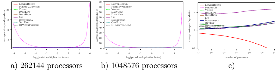
Figure 54: Evaluation of the different heuristics on a Exascale platform with Exponential failures ( MTBF = 1250 years), using Numerical Kernel law with \gamma = 1 , and constant overhead model
