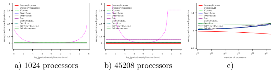
Figure 31: Evaluation of the different heuristics on a Petascale platform with Exponential failures ( MTBF = 500 years), using Numerical Kernel law with \gamma = 1 , and constant overhead model
