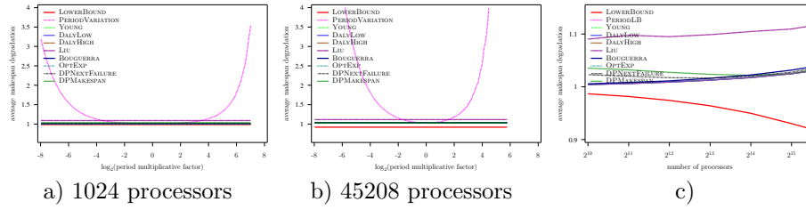
Figure 28: Evaluation of the different heuristics on a Petascale platform with Exponential failures ( MTBF = 125 years), using Numerical Kernel law with \gamma = 0.1 , and constant overhead model
