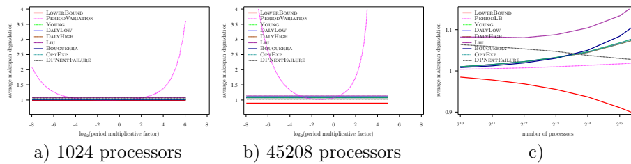
Figure 45: Evaluation of the different heuristics on a Petascale platform with Weibull failures ( MTBF = 500 years), using Numerical Kernel law with \gamma = 10 , and constant overhead model
