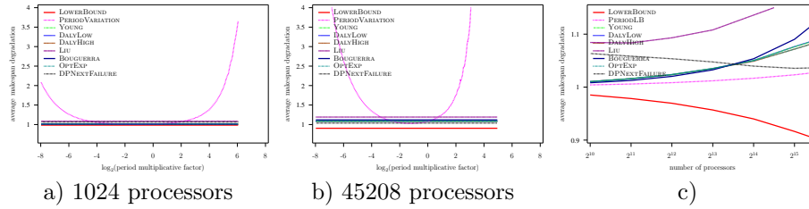
Figure 35: Evaluation of the different heuristics on a Petascale platform with Weibull failures ( MTBF = 500 years), using embarrassingly parallel job, and constant overhead model
