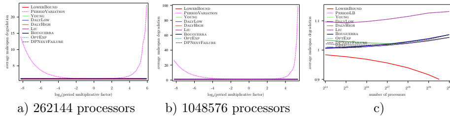
Figure 51: Evaluation of the different heuristics on a Exascale platform with Exponential failures ( MTBF = 1250 years), using embarrassingly parallel job, and constant overhead model
