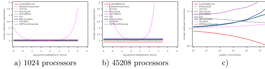
Figure 43: Evaluation of the different heuristics on a Petascale platform with Weibull failures ( MTBF = 500 years), using Numerical Kernel law with \gamma = 1 , and constant overhead model
