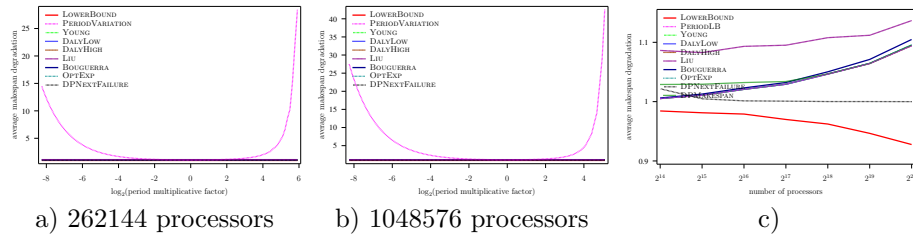
Figure 50: Evaluation of the different heuristics on a Exascale platform with Exponential failures ( MTBF = 1250 years), using Numerical Kernel law with \gamma = 10 , and constant overhead model
