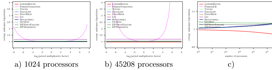
Figure 33: Evaluation of the different heuristics on a Petascale platform with Exponential failures ( MTBF = 500 years), using Numerical Kernel law with \gamma = 10 , and constant overhead model
