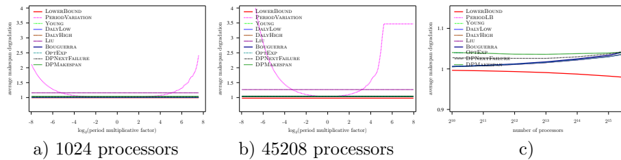
Figure 27: Evaluation of the different heuristics on a Petascale platform with Exponential failures ( MTBF = 500 years), using Amdahl law with \gamma = 10^{-6} , and constant overhead model
