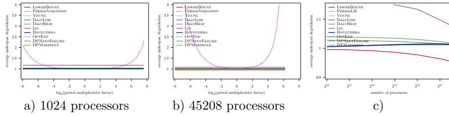
Figure 25: Evaluation of the different heuristics on a Petascale platform with Exponential failures ( MTBF = 500 years) using Amdahl law with \gamma = 10^{-4} , and constant overhead model
