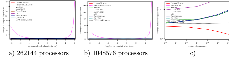
Figure 46: Evaluation of the different heuristics on a Exascale platform with Exponential failures ( MTBF = 1250 years), using embarrassingly parallel job, and constant overhead model
