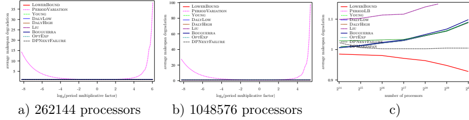
Figure 49: Evaluation of the different heuristics on a Exascale platform with Exponential failures ( MTBF = 1250 years), using Numerical Kernel law with \gamma = 1 , and constant overhead model
