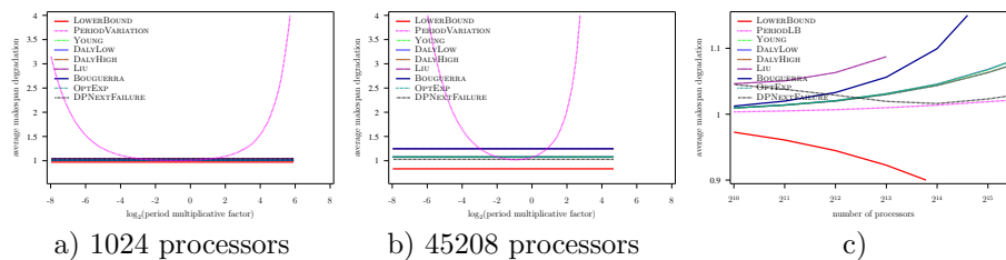
Figure 42: Evaluation of the different heuristics on a Petascale platform with Weibull failures ( MTBF = 125 years), using Numerical Kernel law with \gamma = 1 , and constant overhead model
