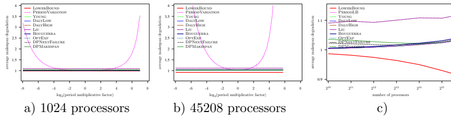
Figure 26: Evaluation of the different heuristics on a Petascale platform with Exponential failures ( MTBF = 125 years), using Amdahl law with \gamma = 10^{-6} , and constant overhead model
