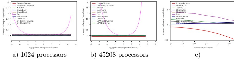
Figure 24: Evaluation of the different heuristics on a Petascale platform with Exponential failures ( MTBF = 125 years) using Amdahl law with \gamma = 10^{-4} , and constant overhead model
