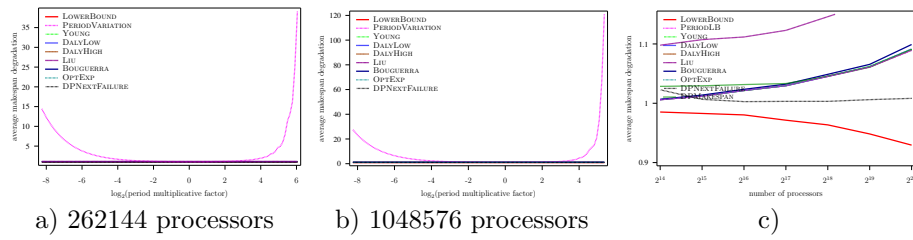
Figure 48: Evaluation of the different heuristics on a Exascale platform with Exponential failures ( MTBF = 1250 years), using Numerical Kernel law with \gamma = 0.1 , and constant overhead model
