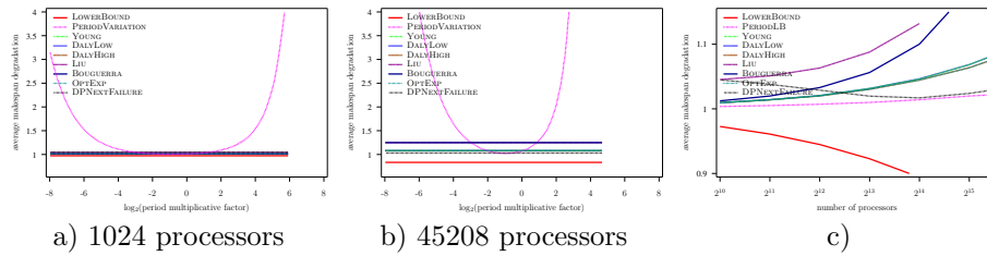
Figure 34: Evaluation of the different heuristics on a Petascale platform with Weibull failures ( MTBF = 125 years), using embarrassingly parallel job, and constant overhead model
