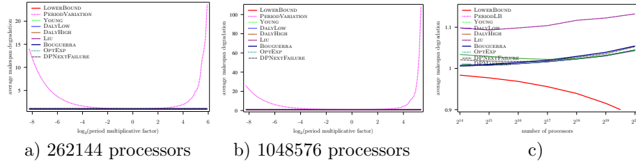
Figure 53: Evaluation of the different heuristics on a Exascale platform with Exponential failures ( MTBF = 1250 years), using Numerical Kernel law with \gamma = 0.1 , and constant overhead model
