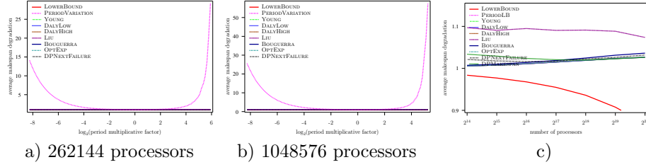
Figure 52: Evaluation of the different heuristics on a Exascale platform with Exponential failures ( MTBF = 1250 years), using Amdahl law with \gamma = 10^{-6} , and constant overhead model
