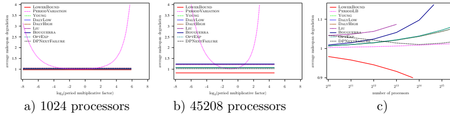
Figure 44: Evaluation of the different heuristics on a Petascale platform with Weibull failures ( MTBF = 125 years), using Numerical Kernel law with \gamma = 10 , and constant overhead model
