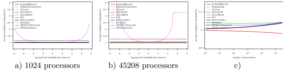
Figure 23: Evaluation of the different heuristics on a Petascale platform with Exponential failures ( MTBF = 500 years) using embarrassingly parallel job, and constant overhead model
