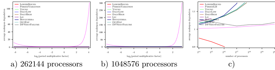
Figure 56: Evaluation of the different heuristics on a Exascale platform with Weibull failures ( MTBF = 1250 years), using embarrassingly parallel job, and constant overhead model
