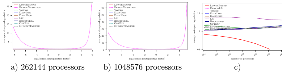
Figure 55: Evaluation of the different heuristics on a Exascale platform with Exponential failures ( MTBF = 1250 years), using Numerical Kernel law with \gamma = 10 , and constant overhead model
