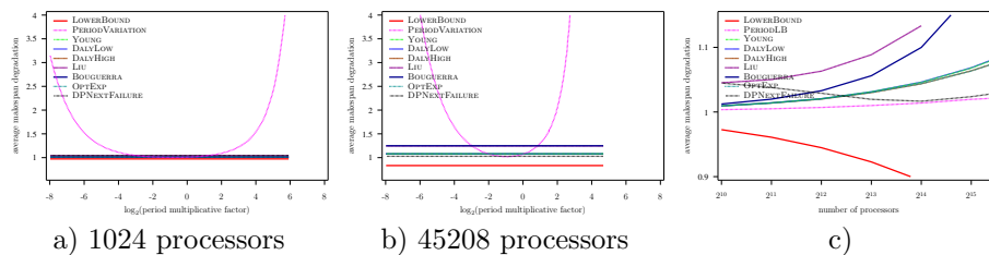
Figure 38: Evaluation of the different heuristics on a Petascale platform with Weibull failures ( MTBF = 125 years), using Amdahl law with \gamma = 10^{-6} , and constant overhead model
