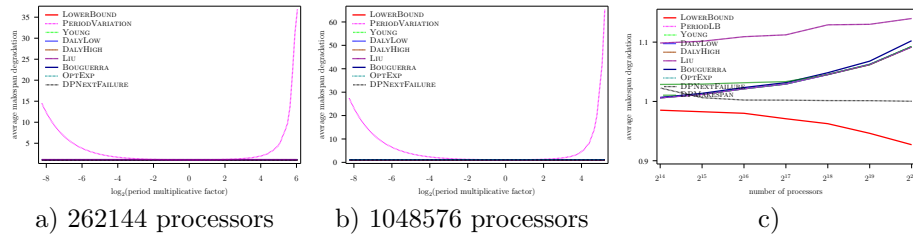
Figure 47: Evaluation of the different heuristics on a Exascale platform with Exponential failures ( MTBF = 1250 years), using Amdahl law with \gamma = 10^{-6} , and constant overhead model
