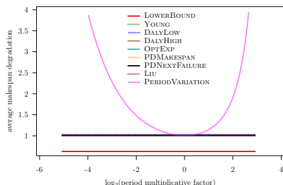
Figure 3: Evaluation of the different heuristics on a single processor with Exponential failures (MTBF = 1 hour).
