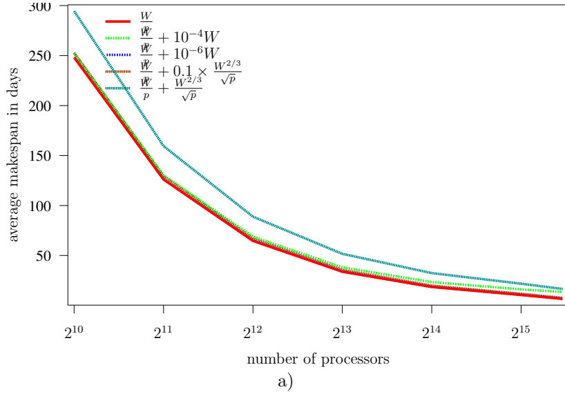
Figure 99: Evolution of the makespan for DPNEXTFAILURE as a function of the platform size for the different application profiles and a constant checkpoint cost (Weibull law, MTBF = 1250 years).
