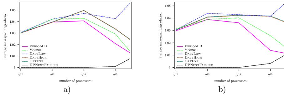
Figure 100: Evaluation of the different heuristics on a Petascale platform with failures based on the failure log of LANL cluster 18 (a) and 19 (b).
