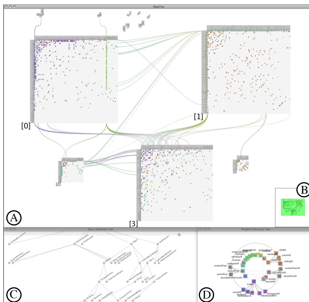
Figure 3: OntoTrix Interface Overview: (A) Main NodeTrix view, (B) Bird's eye view, (C) Class hierarchy view, (D), Property hierarchy view. Visualizing 724 instances (49 classes) and 1 636 object properties (29 definitions) from the NTN ontology.
