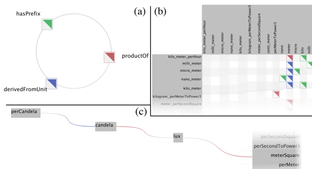
Figure 2: Conveying edge direction: (a) Mapping property type to color hue for units.owl – Semantic Web for Earth and Environmental Terminology; (b) Matrix: milli_meter derives from meter , and has prefix milli ; (c) Node-link: lux is a product of candela and meterSquare , perCandela is derived from unit candela .
