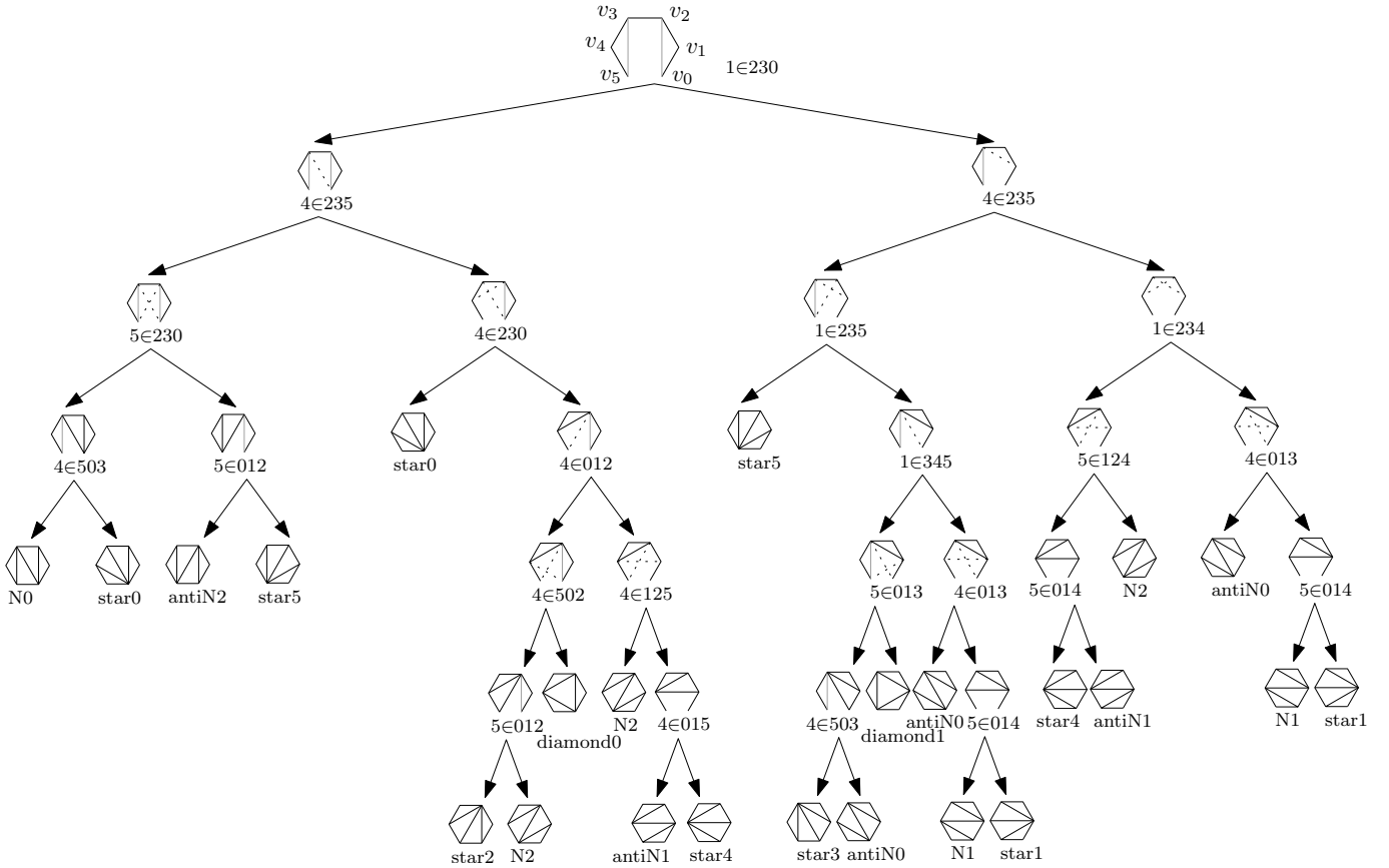
Figure 4: Decision tree for degree 6 deletion.
