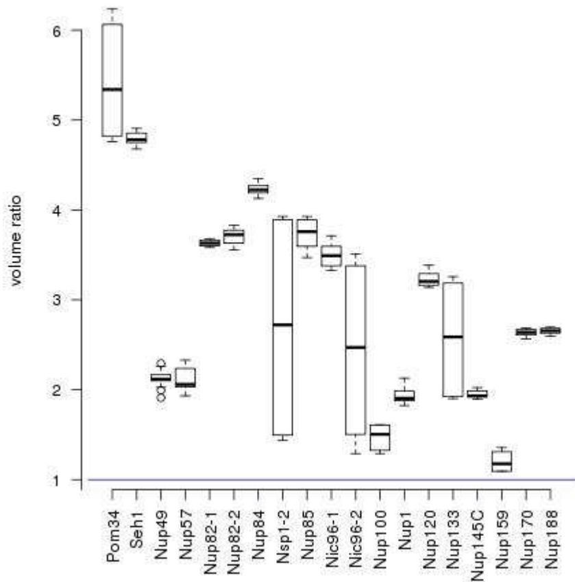
Density maps sorted by reference volumes
