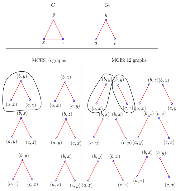
Figure 12: Top. Two labelled graphs G_1 and G_2 . Bottom Left. Maximal Common Edge Sub-graph of G_1 and G_2 (MCES). Bottom Right.: Maximal Common Induced Sub-graph (MCIS) of G_1 and G_2 . If we impose a correspondence between labels ( (a, x), (b, y), (c, z) ), there is one MCES and there are two MCIS—the circled graphs.
