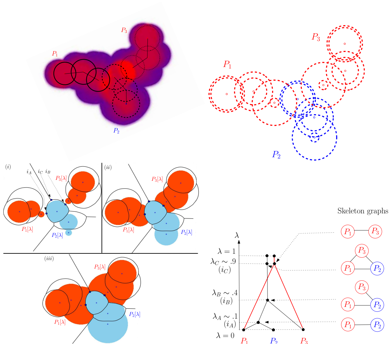
Figure 1: Tracking the interactions of three tolerated proteins of three tolerated balls each. (Top left) Three conformations of three flexible molecules, and a probability density map whose color indicates the probability of a given point to be covered by a random conformation of the ternary complex — from low (blue pixels) to high (red pixels) probabilities. (Top right) The associated bicolor tolerated model, with one blue and two red molecules. Each tolerated molecule consists of a set of pairs of concentric balls, the inner and outer balls. (Bottom left) Sub-figures (i,ii,iii) respectively show grown balls \overline{B}_i[\lambda] for \lambda = 0, 0.5, 1 . The region of the plane consisting of points first reached by a growing tolerated ball is the Voronoi region of this ball, represented by solid lines. Colored solid regions feature the restrictions i.e. the intersection of a growing ball and its Voronoi region. Along the growth process, the restrictions intersect in three points i_A, i_B, i_C , represented as blue squares. (Bottom right) Hasse diagrams encoding contacts between the protein instances. Black tree: all instances; red tree: red instances only.
