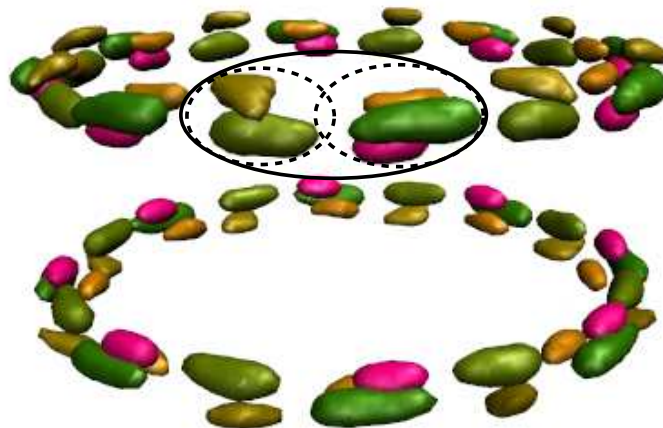
Figure 5: Union of the level-set surfaces from the density maps of protein types of Y -main, at intensity 0.5. The color codes are those of Fig. 2. The circled region illustrates the split of a Y -complex into two pieces (Nup133, Nup84, Nup145C) and (Nup120, Nup85).
