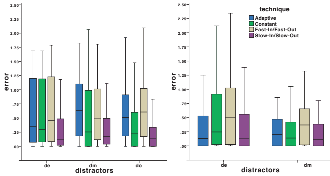
Figure 5. Mean selection error ERROR grouped by distractor profile DISTPROF for all TECH. Generated (left) and real DATASET (right).
