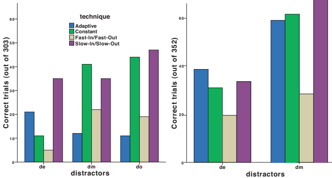
Figure 6. Percent of correct answers grouped by DISTPROF for all TECH. Generated (left) and real DATASET (right).
