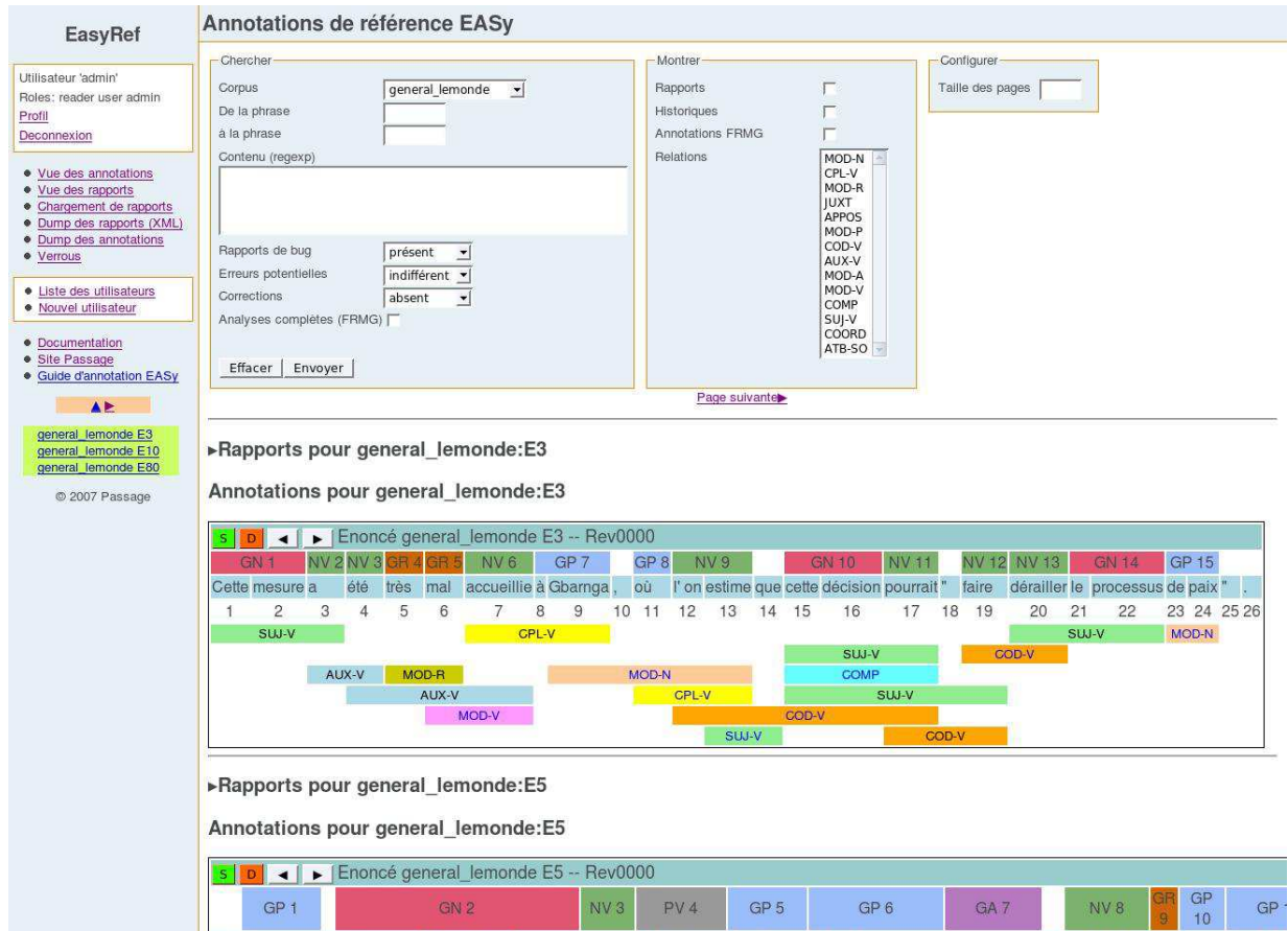
Figure 2: Visualizing annotations with EASYREF
