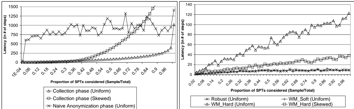
(a) Collection Phase and Naive Anonymization Phase (b) Robust, WM_Soft, WM_Hard Anonymization Phases
