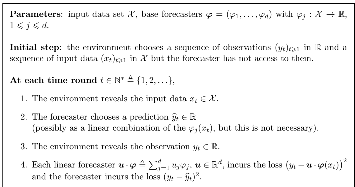
Figure 1: The online linear regression setting.
