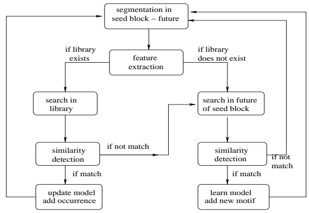
Figure 1: The diagram refers to the single step of the iterative process. At each step the seed block is compared with the models in the library and, if not found, is searched in its near future. At the following step the pair 'seed block-future' shifts of a seed block length along the audio stream and the process is iterated.
