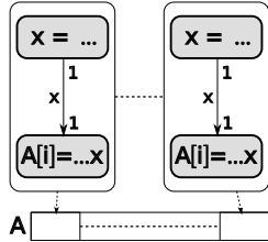
Figure 9: Parallel replicated pipelines with a worksharing construct.
