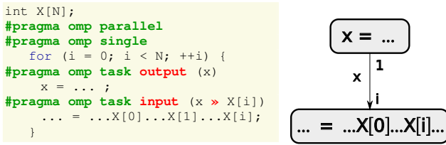
Figure 13: Restricting the horizon size to be a constant does not forbid a task to consume a variable number of elements.
