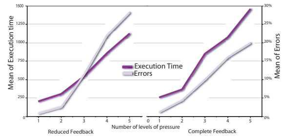
Figure 4. Execution time and errors across N and F
