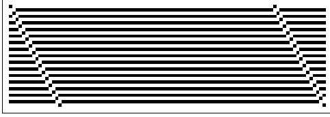
Fig. 3: An example of configurations of CA(3, 3)
