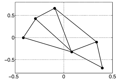
Fig. 10. Selected four triangles to compute the invariant s_{\Delta} .
