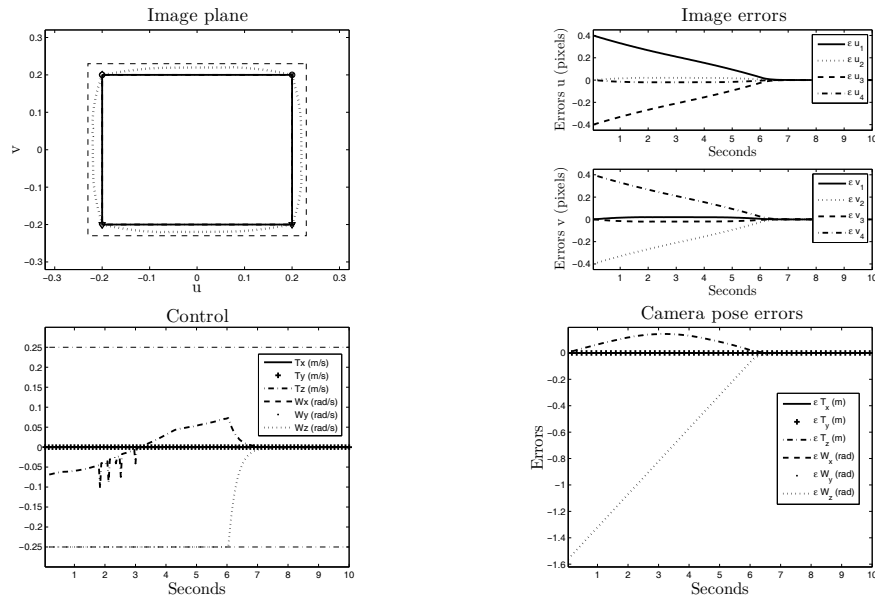
Fig. 20.11 Case 1: VPC_{LM} with N_p = 10 , Q(j) = I and visibility constraint.
