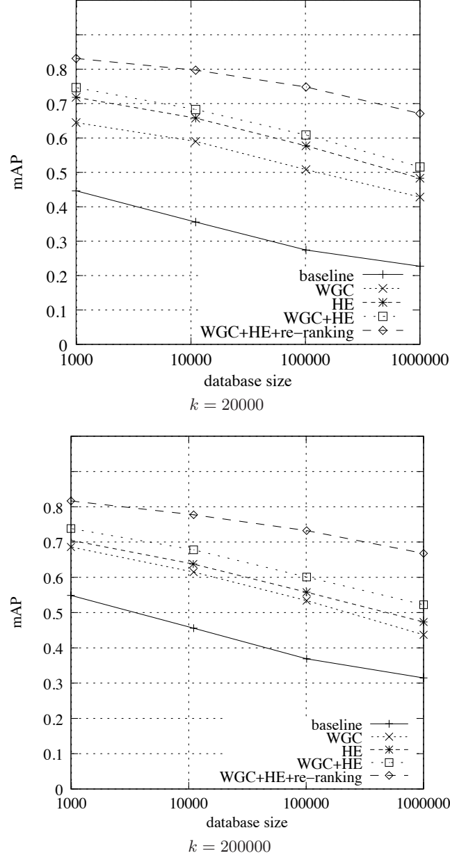
Fig. 10. Performance of the image search as a function of the dataset size for BOF, WGC, HE ( h_t = 22 ), WGC+HE, and WGC+HE+re-ranking with a full geometrical verification (shortlist of 100 images). The dataset is Holidays with a varying number of distractors from Flickr1M .
