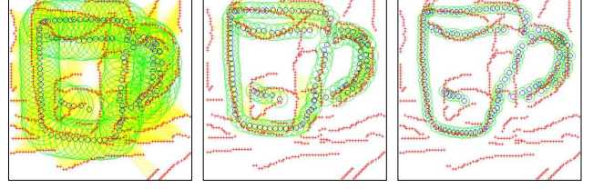
TPS-RPM with class-specific shape constraints
