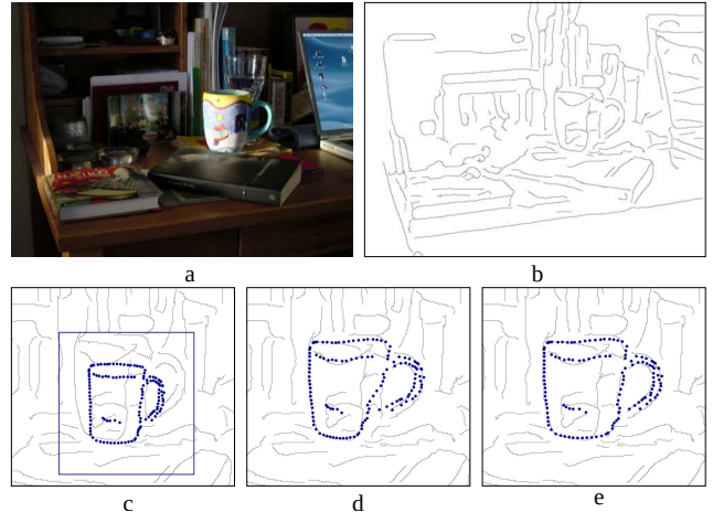
Fig. 8 Object detection. (a) A challenging test image and its edgemap b). The object covers only about 6% of the image surface, and only about 1 edgel in 17 belongs to its boundaries. (c) Initialization with a local maximum in Hough space. (d) Output shape with unconstrained TPS-RPM. It recovers the object boundaries well, but on the bottom-right corner, where it is attracted by the strong-gradient edges caused by the shading inside the mug. (e) Output of the shape-constrained TPS-RPM. The bottom-right corner is now properly recovered.
