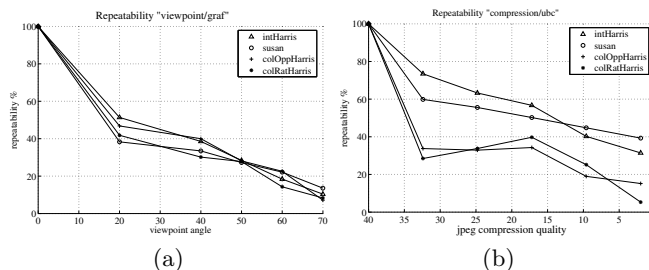
Fig. 2. Repeatability for different detectors on the viewpoint set (a) and the compression set (b)
