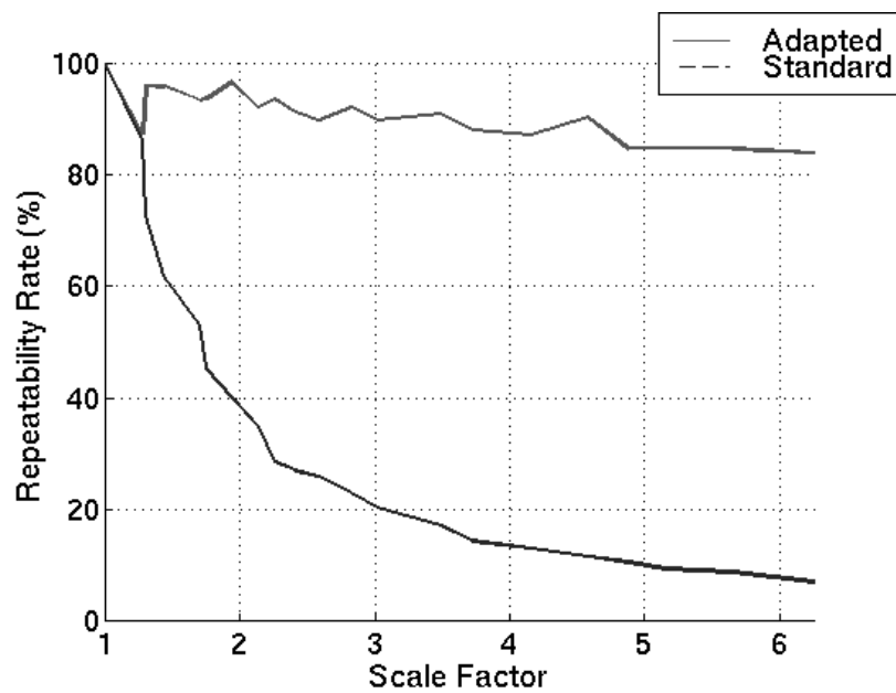
Figure 3: Comparison of the standard Harris detector ( Standard or bottom curve) and the scale-space version ( Adapted or top curve). The comparison criteria is the repeatability rate which is displayed as a function of the scale factor.
