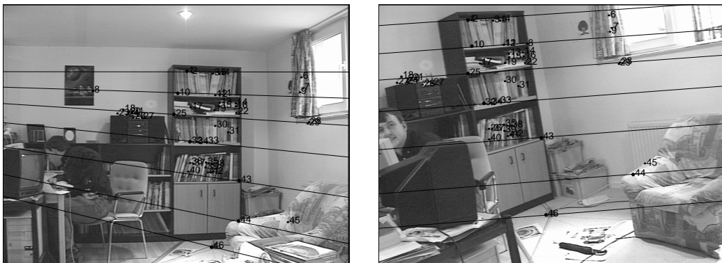
Figure 12: This figure shows the epipolar geometry as computed with the matching and estimation method described in this paper. Notice the large discrepancy in the viewpoints associated with the two images. The matcher seems to give advantage to collections of coplanar points.
