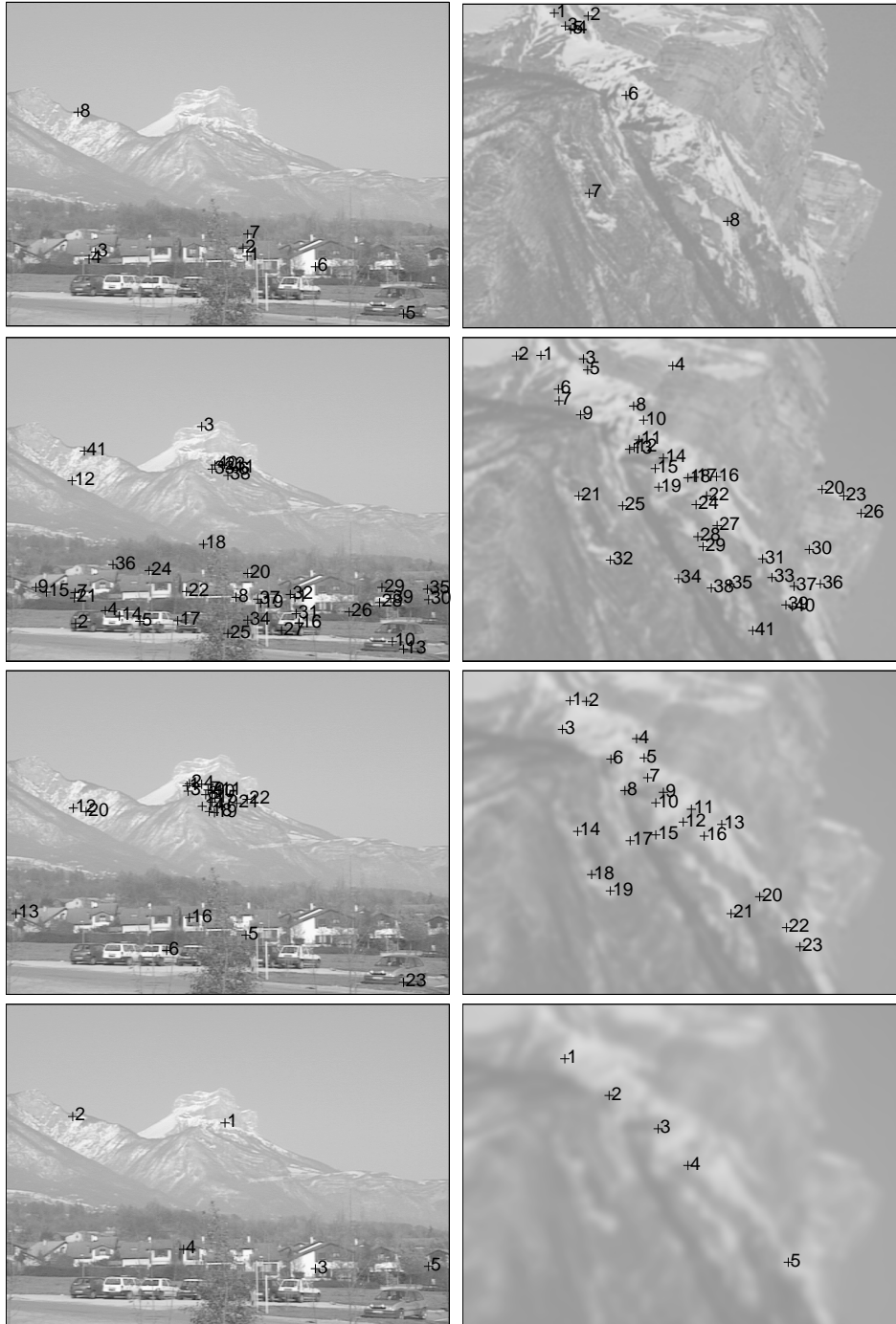
Figure 7: Initial point-to-point assignments obtained at four scales (1,3,5,8). The true resolution factor between the two images is 5.
