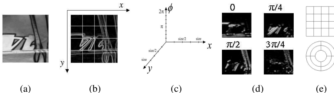
Fig. 1. SIFT descriptor. (a) Detected region. (b) Gradient image and location grid. (c) Dimensions of the histogram. (d) 4 of 8 orientation planes. (e) Cartesian and the log-polar location grids. The log-polar grid shows 9 location bins used in shape context (4 in angular direction).
