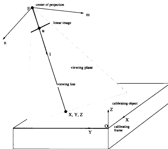
Fig. 1. A general view of a linear camera, a calibrating object, and their associated frames.
