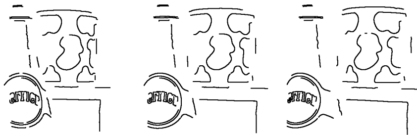
Fig. 8. Three view matching. 25 contour chains are matched. There is only one incorrect match which arises from a specularity on the bottle.
