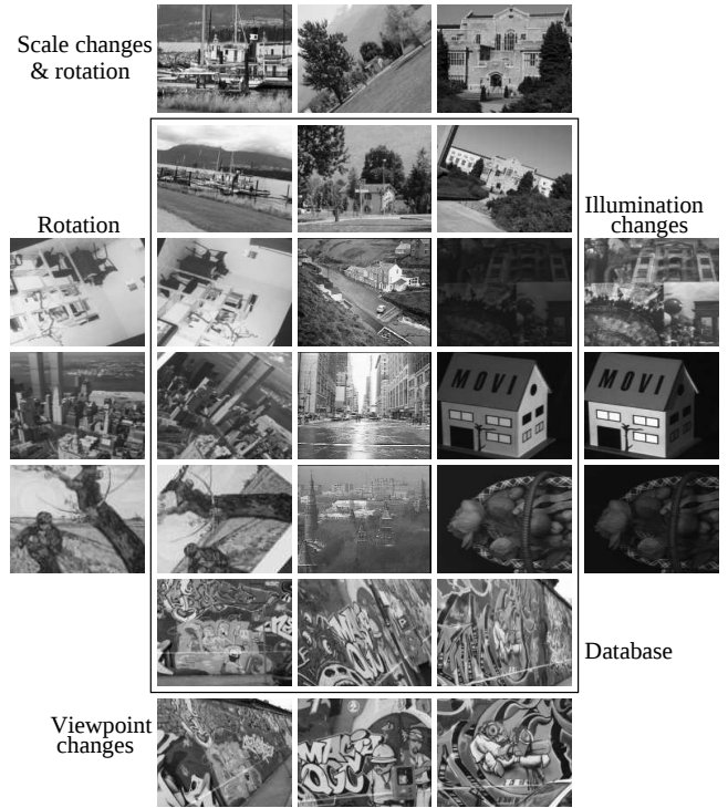
Figure 5: Test images.
