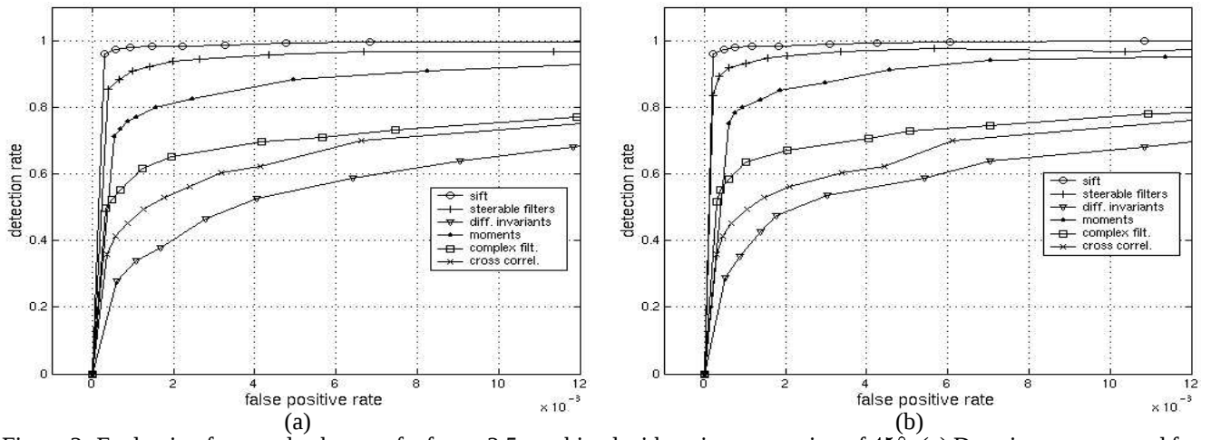
Figure 2: Evaluation for a scale change of a factor 2.5 combined with an image rotation of 45°. (a) Descriptors computed for Harris-Laplace points. (b) Descriptors computed for DoG points.
