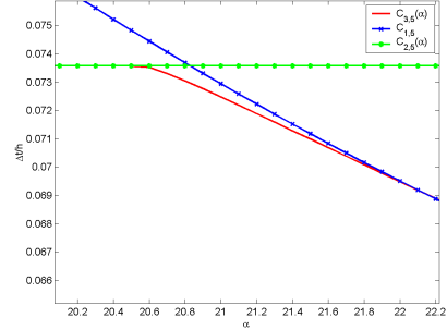
Figure 11: Zoom on the 3 cond. for
