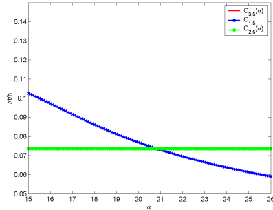
Figure 10: The 3 conditions for p = 5 p = 5
