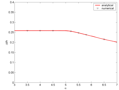
Figure 12: Numerical comparison in P^1 Figure 13: Numerical comparison in P^2
