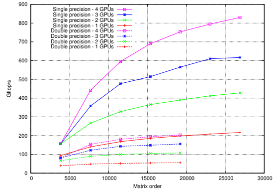
Figure 6. Scalability of the BF-LL variant on Opteron-Tesla.
