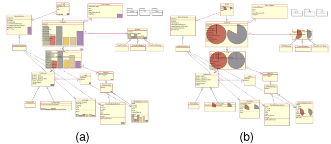
Fig. 18. (a) MetricView height bars (b) MetricView pie charts
