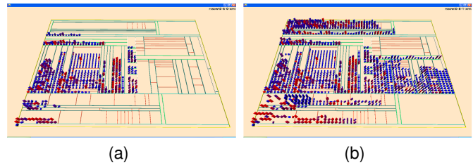
Fig. 29. Visualization of evolution with VERSO from [53].
