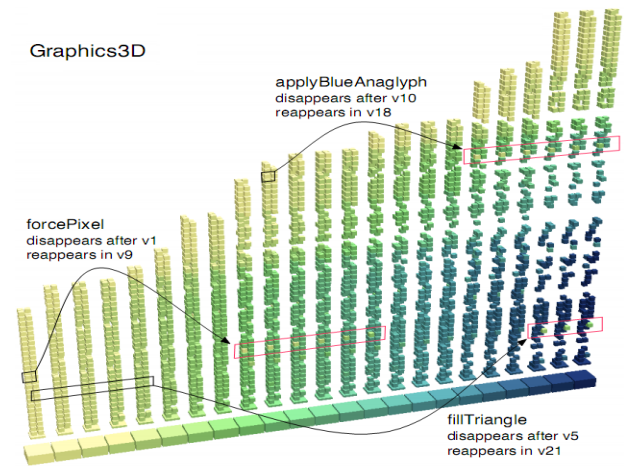
Fig. 26. Timeline from [48]: evolution of the "Graphics3D" class of the Jmol software
