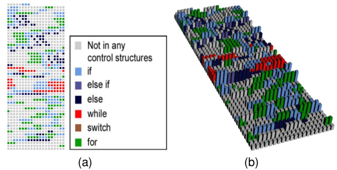
Fig. 1. (a) SeeSoft and (b) sv3D from [3].
