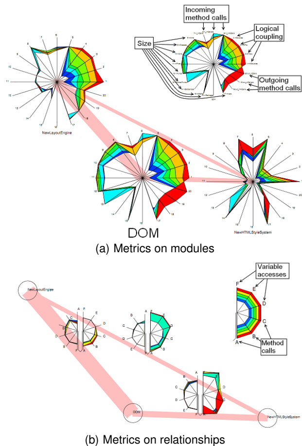
Fig. 31. RelVis from [52] (modified)
