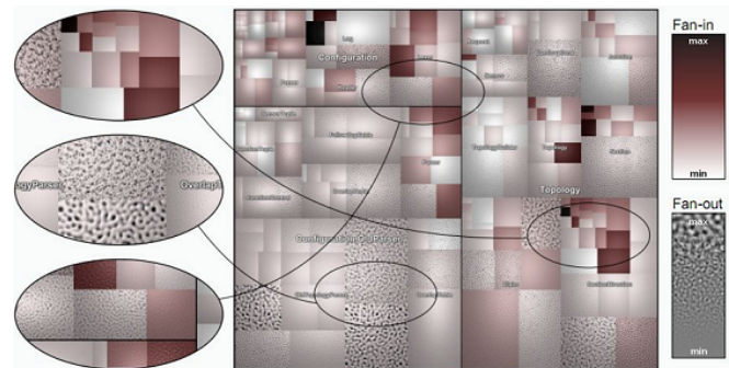
Fig. 21. Treemap with color and texture from [39].
