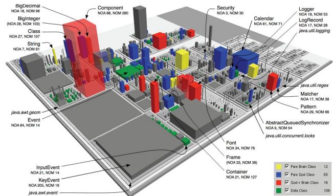
Fig. 23. CodeCity class-level disharmonies map from [43].
