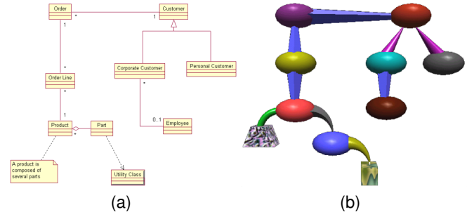
Fig. 10. (a) UML diagram (b) equivalent geon diagram.
