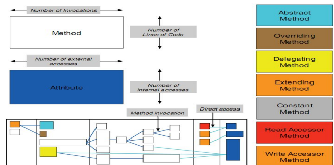
Fig. 2. Class Blueprint from [92].
