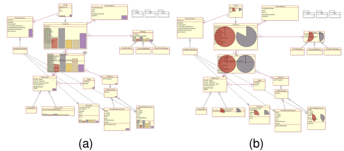
Fig. 18. (a) MetricView height bars (b) MetricView pie charts
