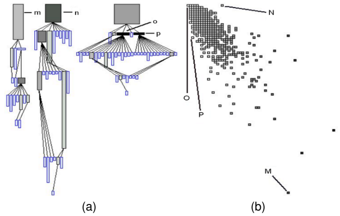
Fig. 20. Polymetric views from [36]: (a) Inheritance Tree and (b) Correlation graph.
