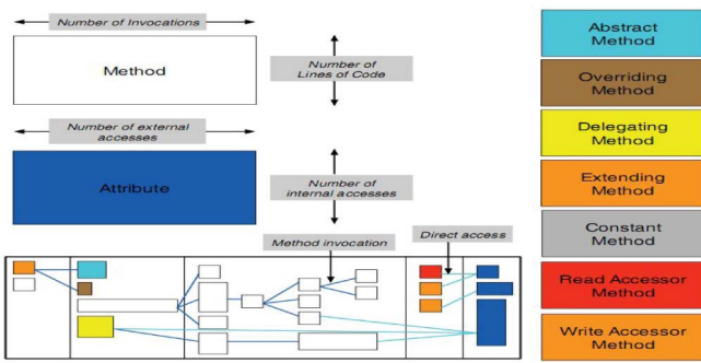
Fig. 2. Class Blueprint from [92].
