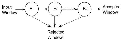
Fig. 5 Cascade of boosted classifiers.
