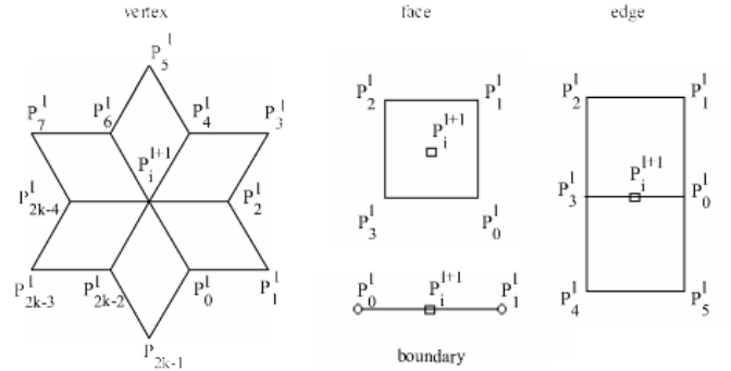
Figure 6. Linear constraints are generated on coarse levels using the Catmull-Clark masks according to the expression listed in Table 1.
