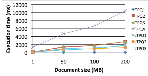
Fig. 10. Scalability of view-based query evaluation.
