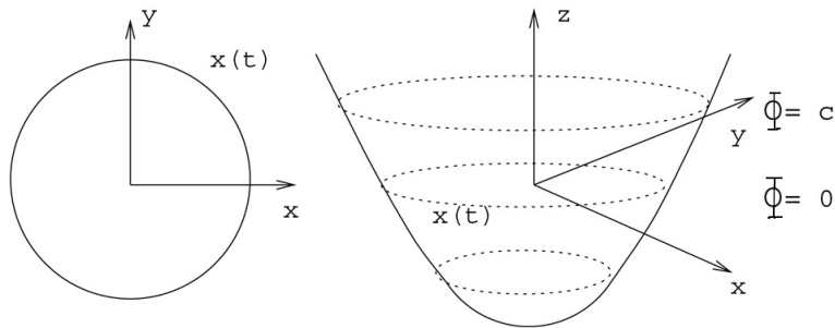
Figure 3: At each time t the propagating front x(t) is the zero level set of a function \Phi(x(t), t) solution of a Hamilton-Jacobi equation.
