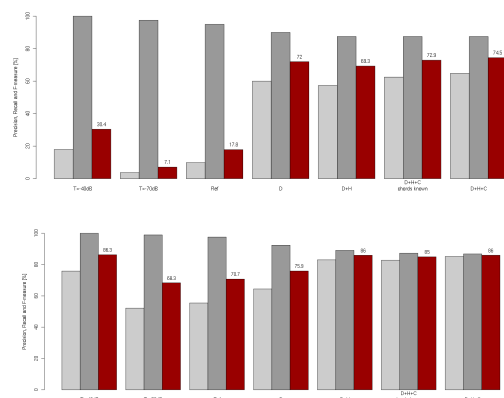
Figure 12: Results for 7 different models obtained for RWC-C24A (top, \alpha = 2.3 , L = 12 , N = 70 ) and RWC-C22 (bottom, \alpha = 1.3 , L = 12 , N = 75 ).
