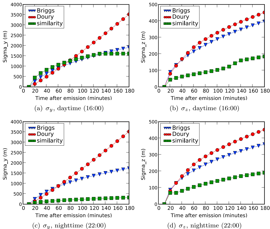
Figure 8. Evolution of the (a and c) horizontal standard deviation \sigma_y , and (b and d) vertical standard deviation \sigma_z , during 3 h, for the three parameterizations and two puff release times. Figures 8a and 8b denote a puff emitted at the beginning of emission (1600 UTC). Figures 8c and 8d denote a puff emitted during the night (2200 UTC). The stability class is D (neutral).
