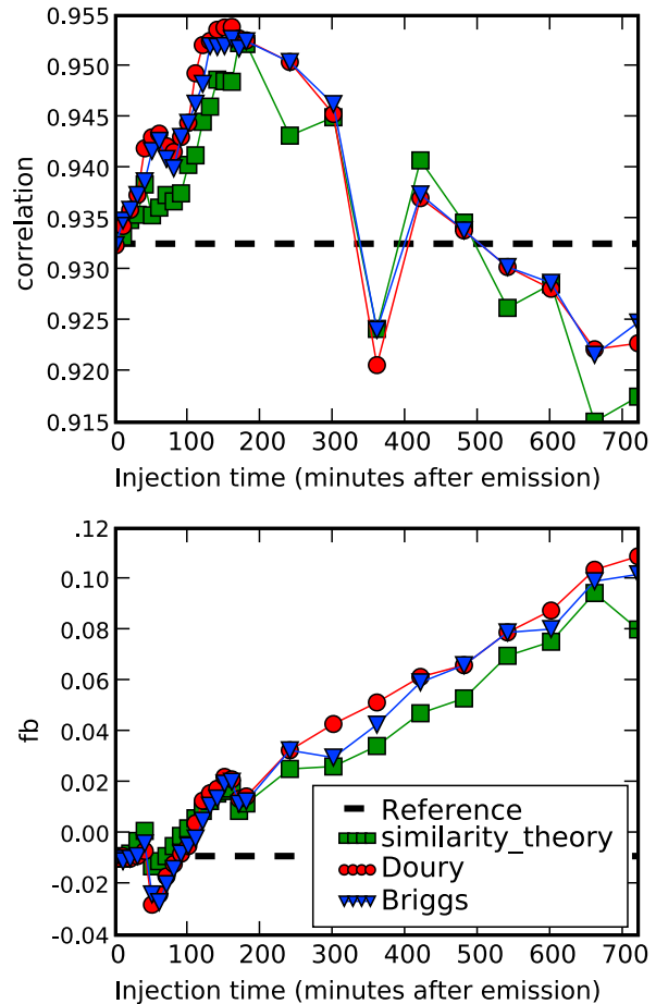
Figure 12. Evolution of the (top) correlation and (bottom) fractional bias for arrival times at stations, against the puff injection time. The simulations are carried out with the column injection for all three Gaussian parameterizations.
