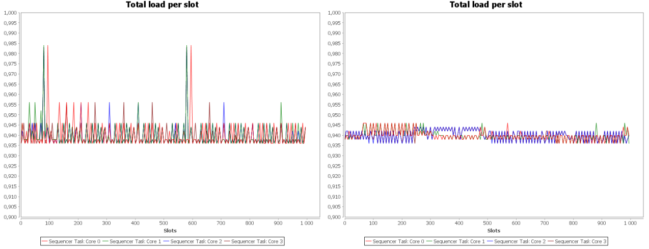
Figure 2: A set of runnables corresponding to slightly less than 94% of CPU load scheduled on a 4-core ECU with LL (left-hand graphic) and G-LL 1σ (right-hand graphic). Graphics obtained from RTaW NETCAR-ECU.
