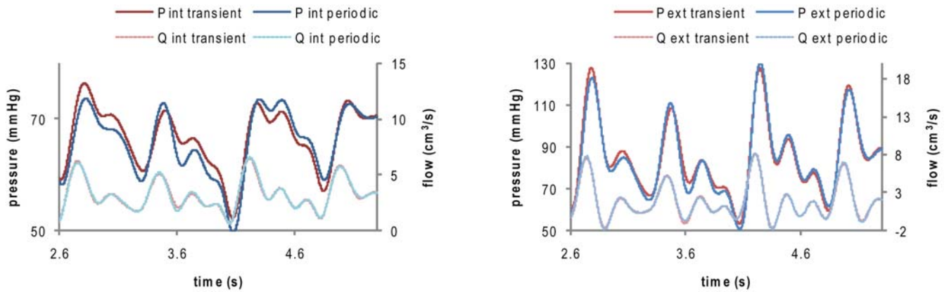
Figure 18: Comparison of flow and average pressure at the outlet boundary for the periodic RCR boundary condition and the fully transient RCR boundary condition in a carotid bifurcation with a stenosis in the internal side. Left plot: internal carotid. Right plot: external carotid.
