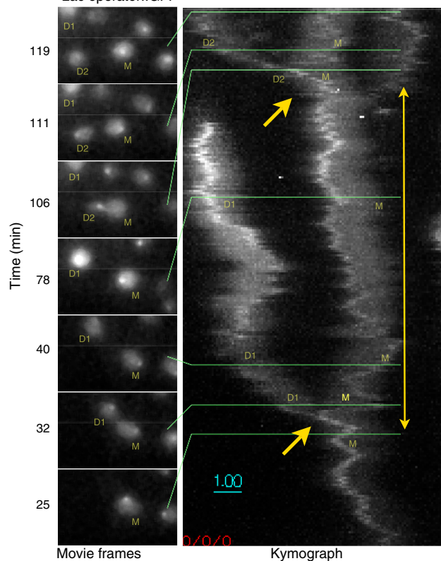
Fig. 7. At low light levels ( I = 5 \times 10^{-4}I_0 ), dense-regime imaging can continue for 2 h, encompassing a whole cell cycle, without fading or loss of viability. The entire series is shown in the SI Text . At left, individual frames from the 2 h imaging sequence, centered on the original cell, are shown proceeding in time from bottom to top. YDB271 yeast cells are labeled M (original mother cell), D1 (first daughter cell), and D2 (second daughter cell). Right, a kymograph created by averaging the 3D stacks in 30 s groups, then projecting the maximum intensity of the time-averaged 3D stacks first along the Z axis, then along the Y axis. Cell divisions are indicated by single arrows; the two-headed arrow delimits an entire cell cycle of the mother cell.
